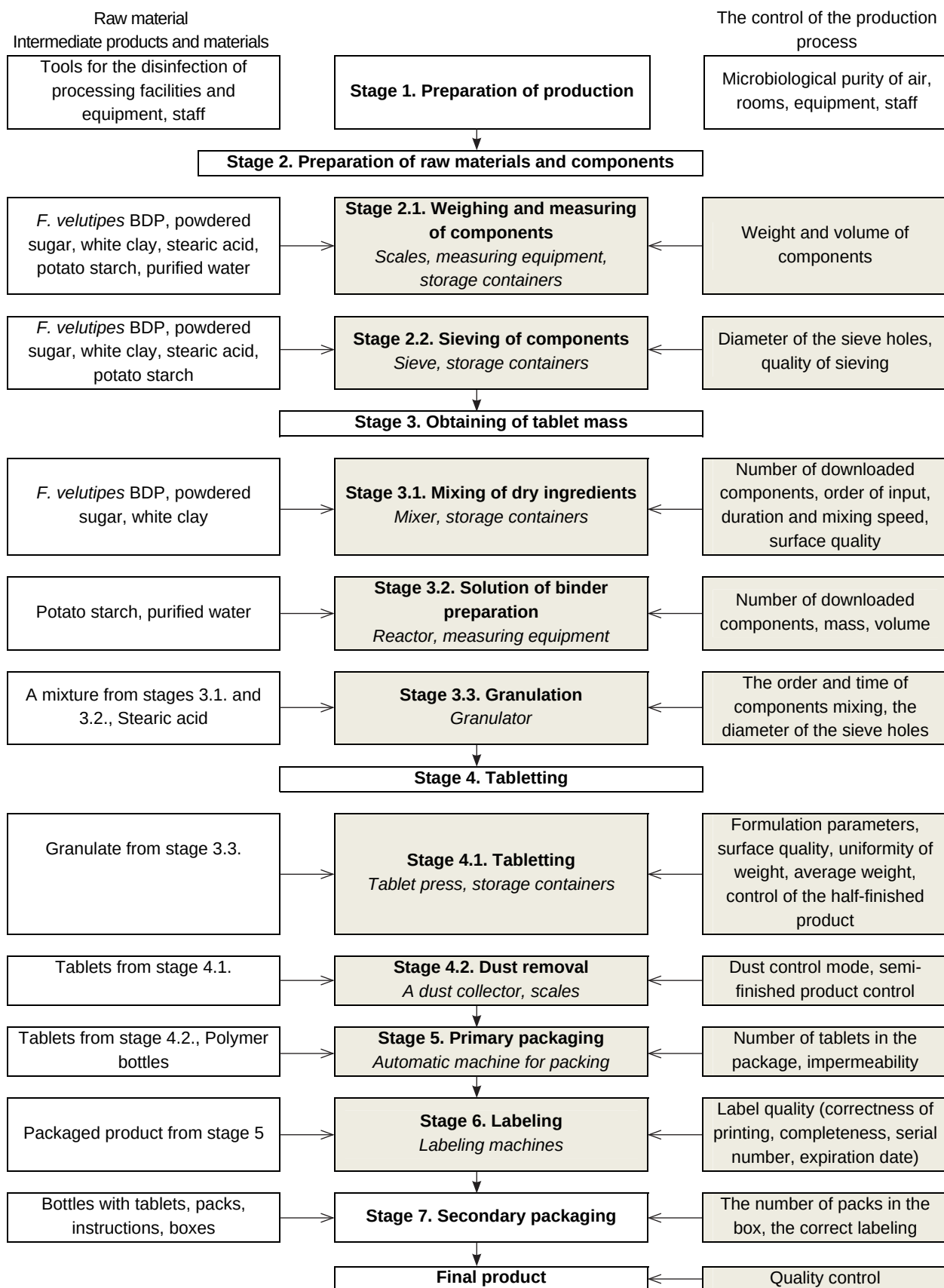
Figure 1. The technological block diagram of tablets based on F. velutipes BDP production
